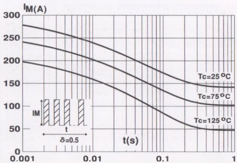
Fig.5 : Non repetitive surge peak forward current versus overload duration. (BYW81P)
