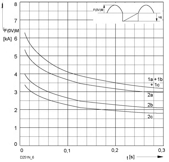
Bild / Fig. 4 Grenzstrom / Maximum overload forward current I_{F(0V)M} = f(t) 1 - I_{FAV(vor)} = 0\text{ A} ; t_{vj} = t_c = 25\text{ °C} 2 - I_{FAV(vor)} = 1\text{ A} ; t_c = 100\text{ °C} ; t_{vj} = 100\text{ °C} a - V_R \leq 50\text{ V} b - V_R = 0,5 V_{RRM} c - V_R = 0,8 V_{RRM}
