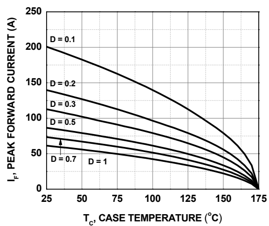
Figure 4. Current Derating
