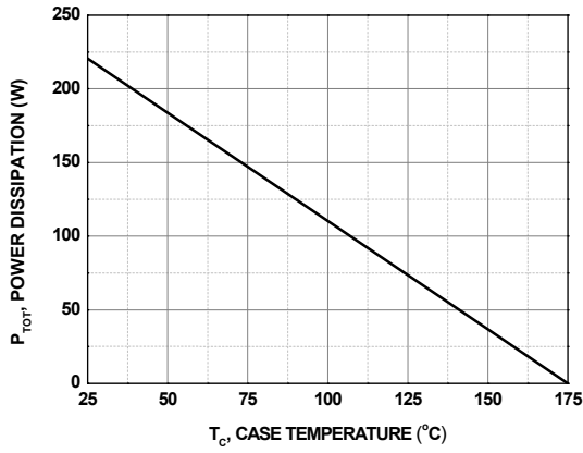
Figure 5. Power Derating
