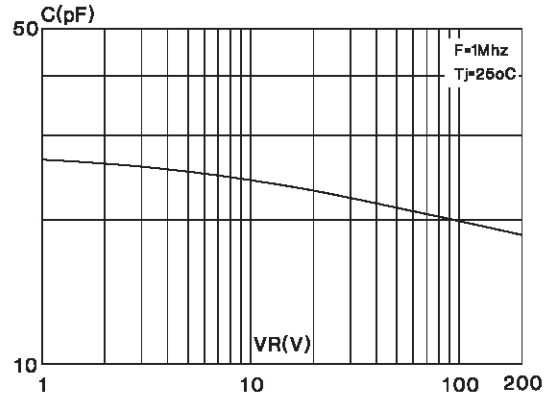
Fig.10 : Junction capacitance versus reverse voltage applied (Typical values) (Per diode).
