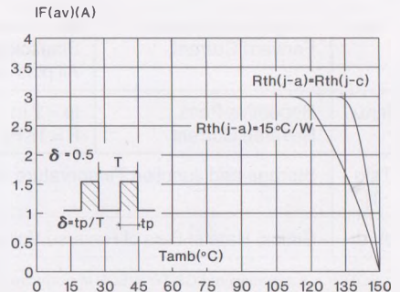
Fig. 2 : Average current versus ambient temperature.
