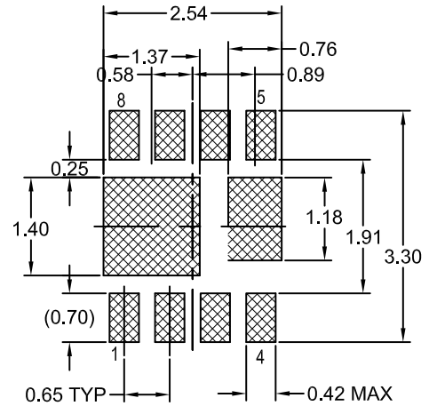
RECOMMENDED LAND PATTERN (NSMD PAD TYPE)
