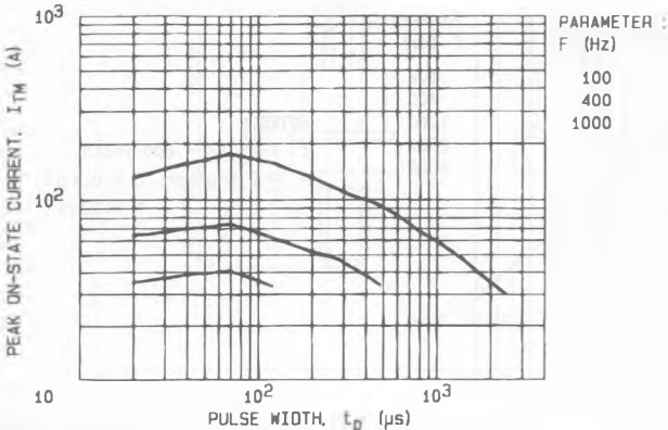
FIG. 6 - MAXIMUM ALLOWABLE PEAK ON-STATE CURRENT VERSUS PULSE WIDTH FOR T 0 = 80 °C.
