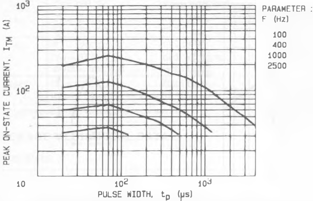
FIG. 5 - MAXIMUM ALLOWABLE PEAK ON-STATE CURRENT VERSUS PULSE WIDTH FOR T 0 = 85 °C.
