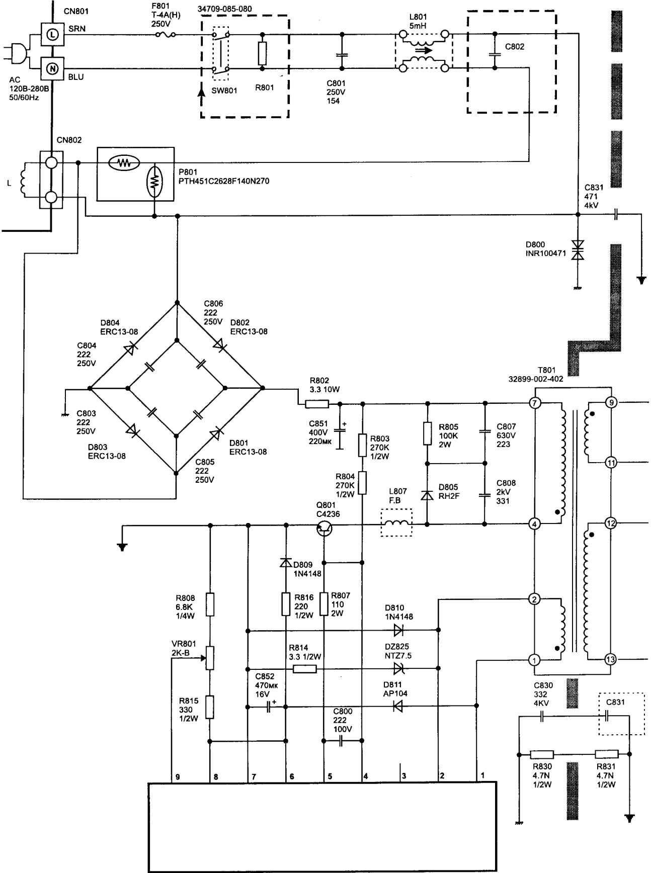
IC801 CDH209B
